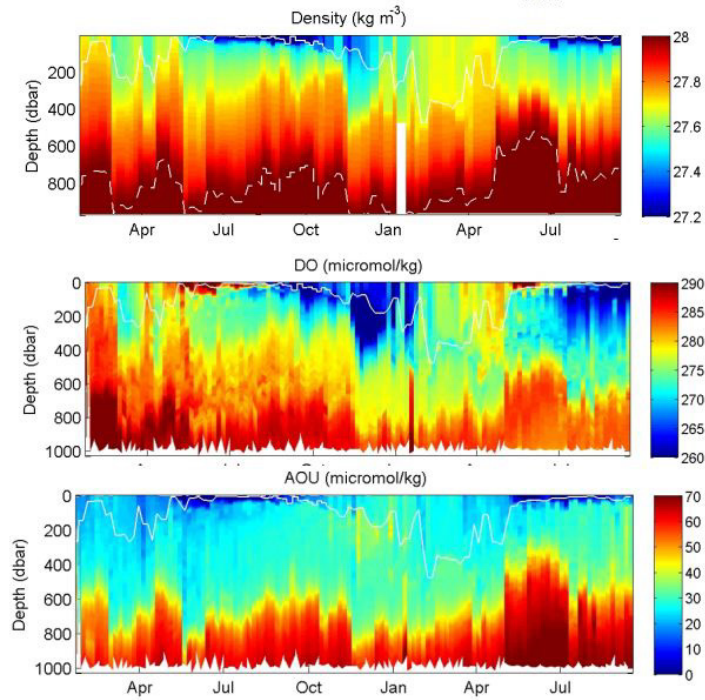
Figure 2.3.1: Density dissolved oxygen and apparent oxygen time series ( \text{AOU} = [\text{O2}]_{\text{sat}} - [\text{O2}] ), Jan2014-Sept2015).
