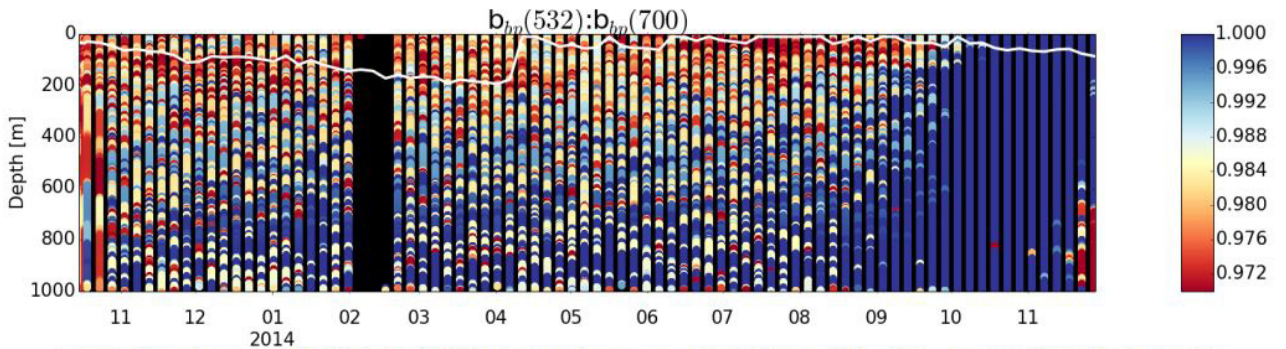
Figure 2.3.2: To first order \text{bbp}(532):\text{bbp}(700) decreased as a function of depth suggesting that small particles become more abundant in the mesopelagic zone.
